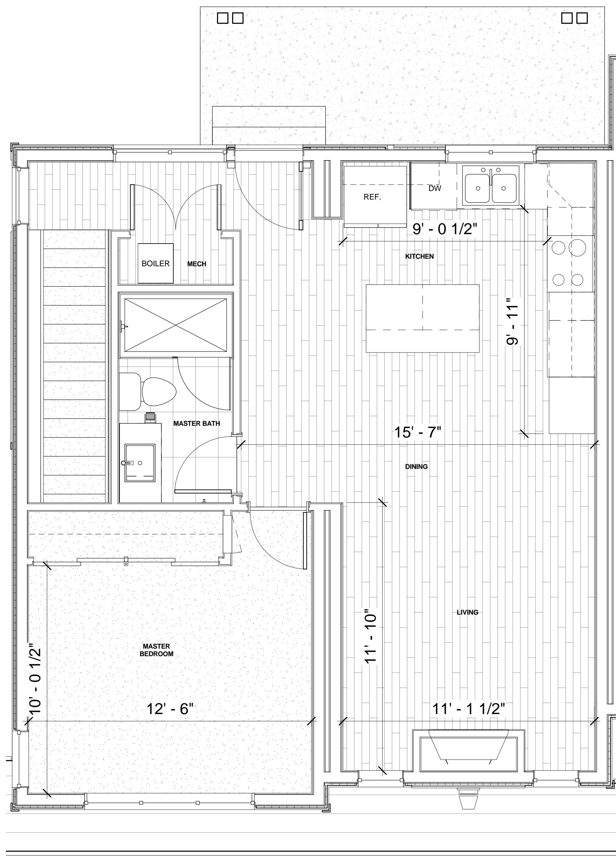
2 UNIT 2.1 A - LEVEL 02 - PLAN DIMENSIONS 3/8" = 1'-0"
