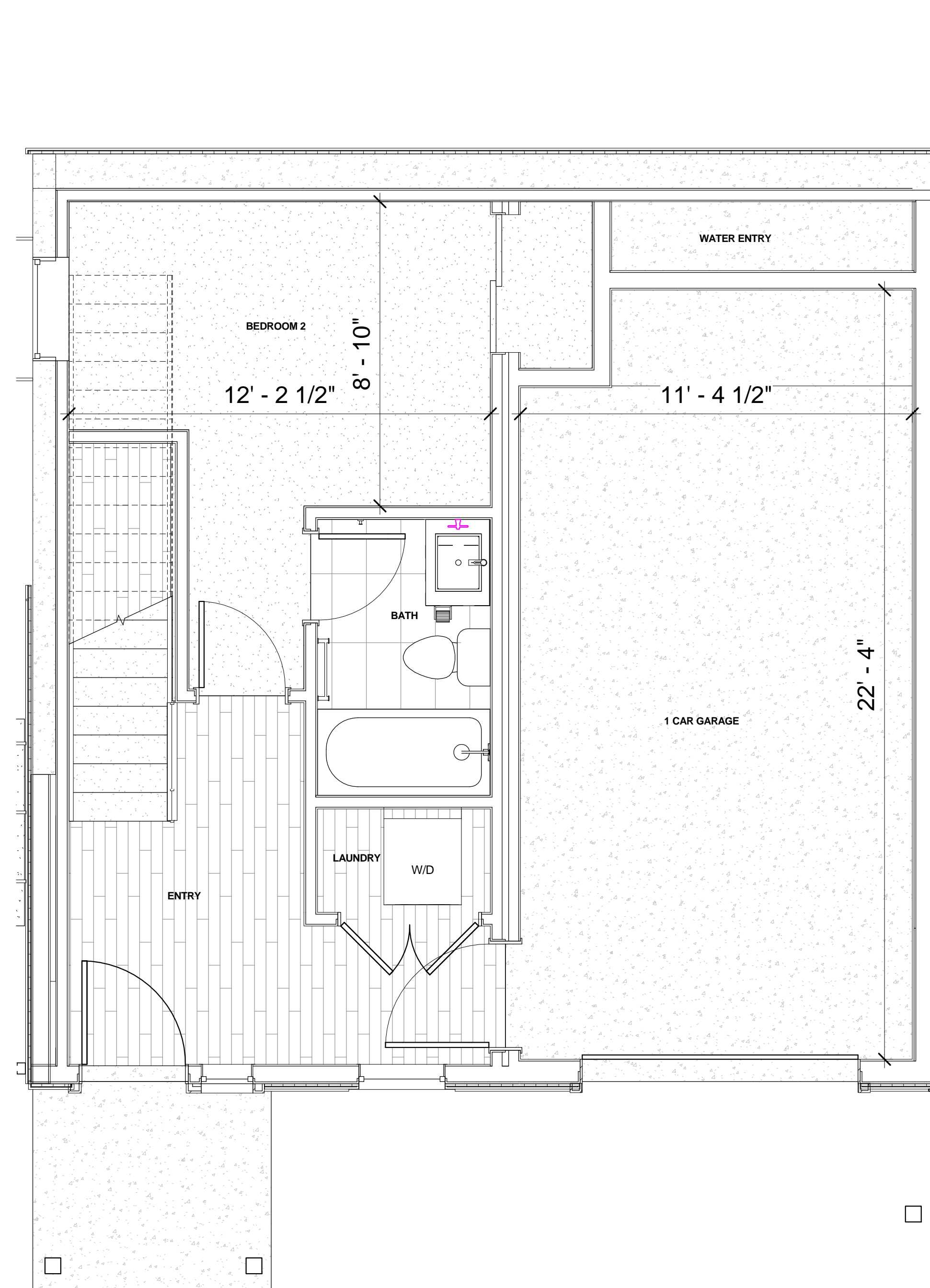
1 UNIT 2.1 A - LEVEL 01 - PLAN DIMENSIONS 3/8" = 1'-0"
