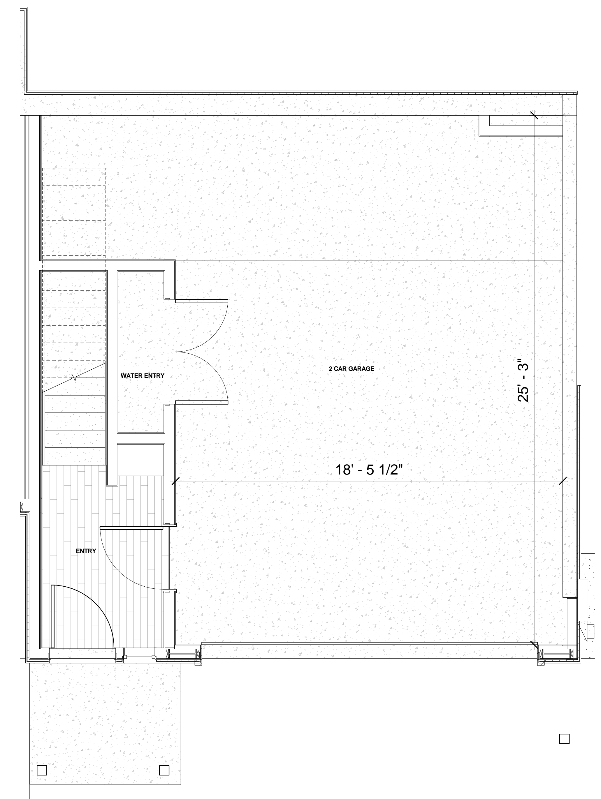
1 UNIT 2.2 A - LEVEL 01 - PLAN DIMENSIONS 3/8" = 1'-0"
