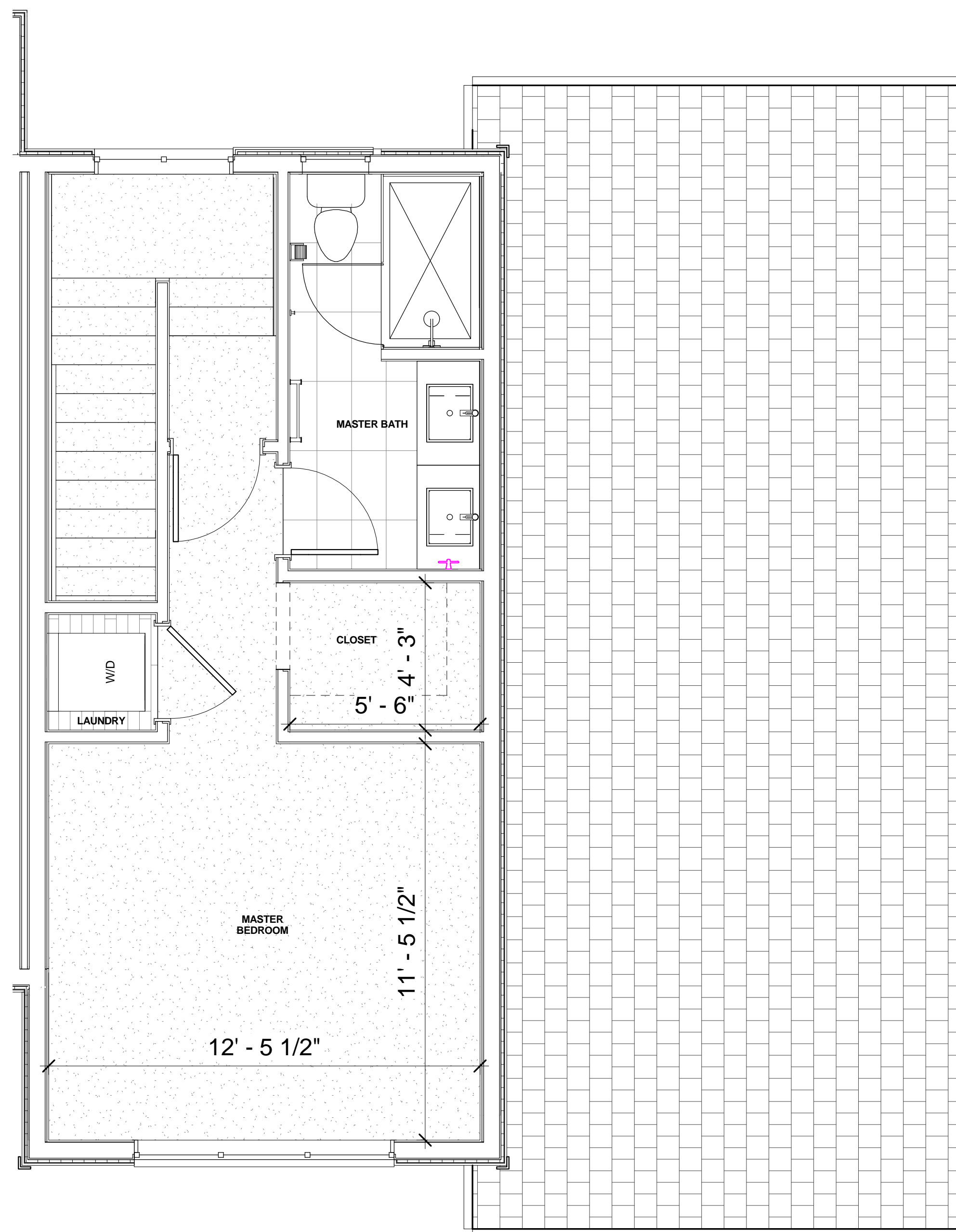
3 UNIT 2.2 A - LEVEL 03 - PLAN DIMENSIONS 3/8" = 1'-0"
