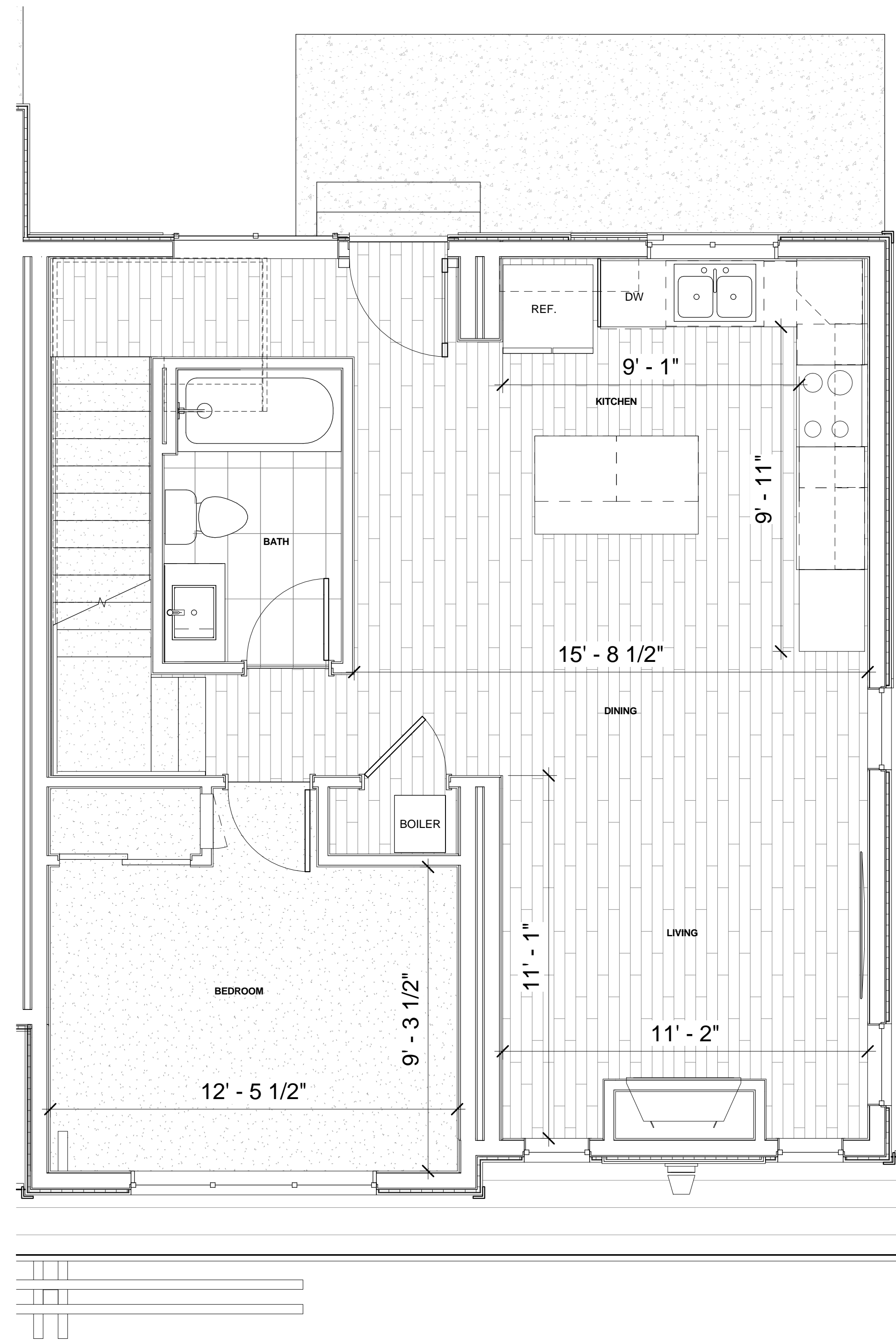
2 UNIT 2.2 A - LEVEL 02 - PLAN DIMENSIONS 3/8" = 1'-0"
