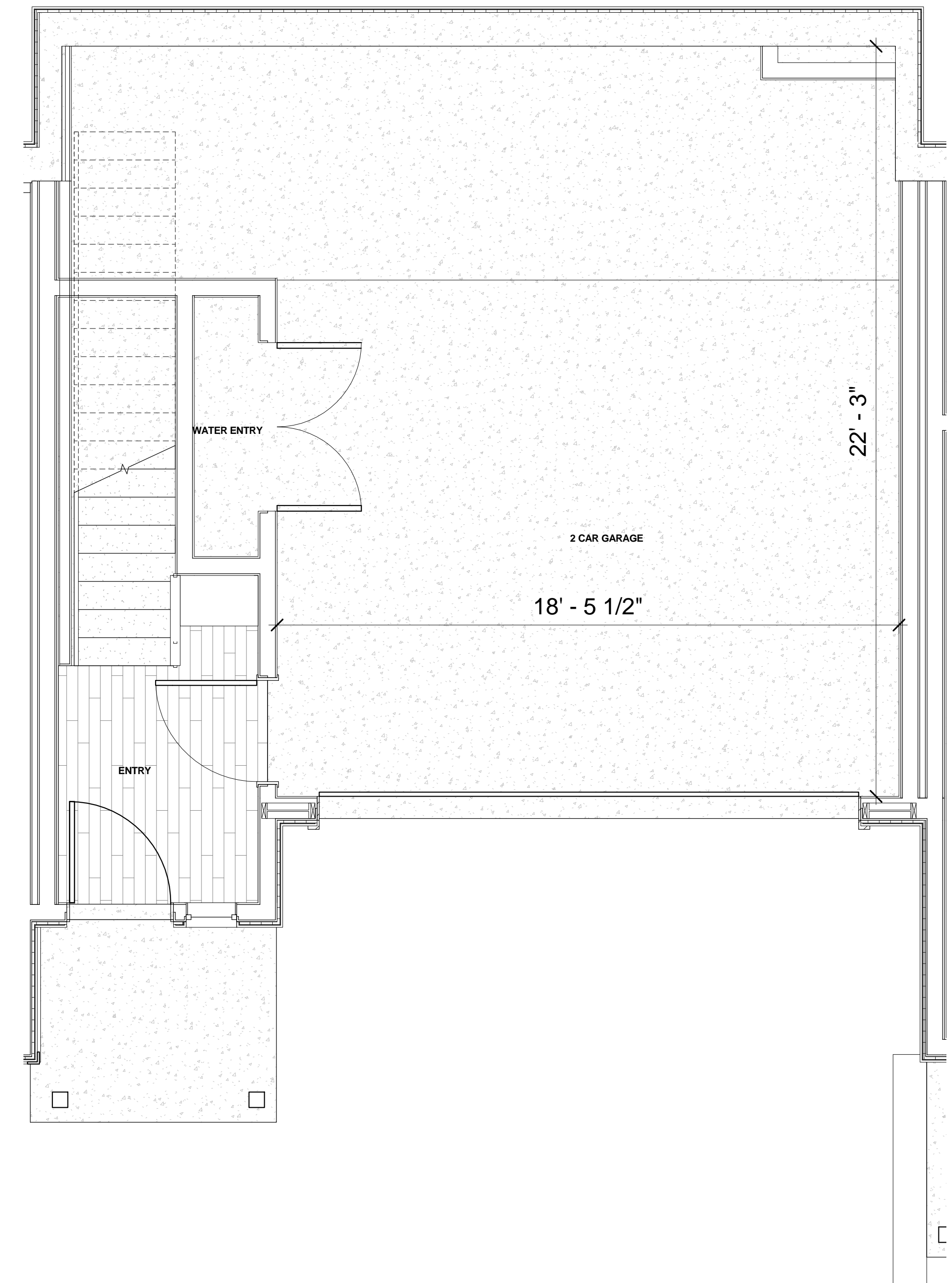
1 UNIT 3.2 A - LEVEL 01 - PLAN DIMENSIONS 3/8" = 1'-0"
