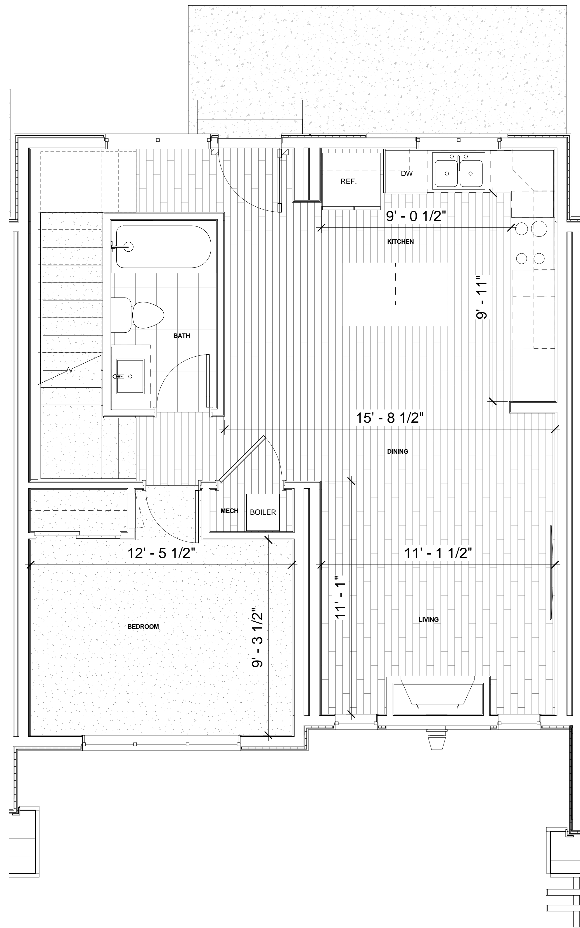
2 UNIT 3.2 A - LEVEL 02 - PLAN DIMENSIONS 3/8" = 1'-0"
